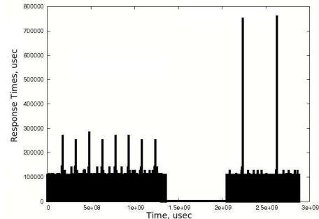
Fig.1: NAND Flash device delays
